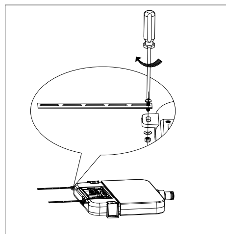
INSTALLATION OF SUSPENSION BAR
